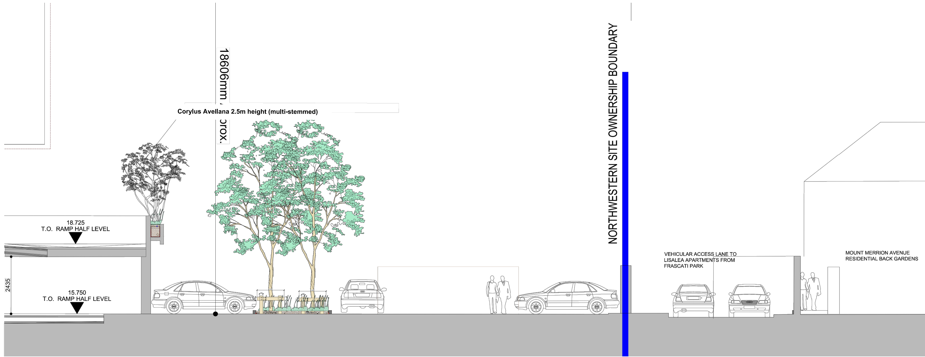
CONSTRUCTION SECTION CS-04 - THROUGH PODIUM PLANTERS AND NORTH-WESTERN BOUNDARY/ Scale 1:100
